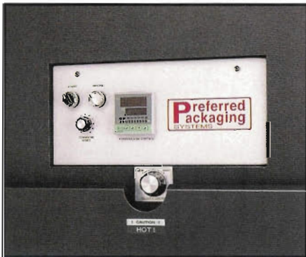
Tunnel Controls
